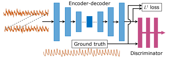
Figure 11: VS-Net for merging and refining vital signs waveform, with an encoder-decoder architecture.
