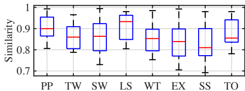
Figure 24: Heartbeat monitoring performance on 77 GHz radar under different body movements.
